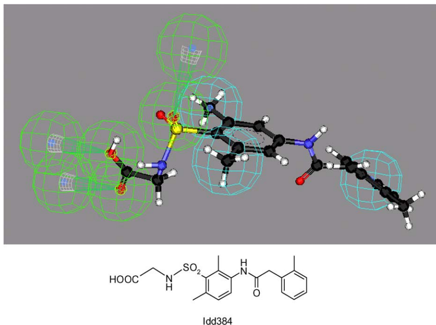
Figure 2. Pharmacophore model representing the interactions of Idd384 with the ALR2 active site.
