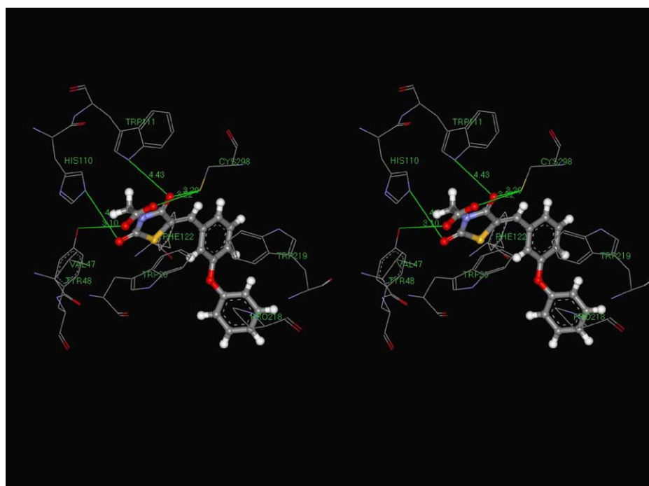
Figure 5. Possibilities of hydrogen bond interactions of docked inhibitor 4a in the ALR2 active site.
