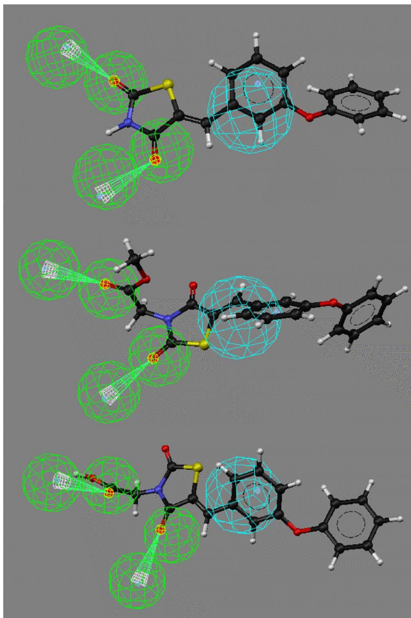
Figure 3. Compounds 2a , 3a and 4a (from the top to the bottom) mapped on a common features pharmacophore model (Green: H bond acceptor; Cyan: lipophilic region).
