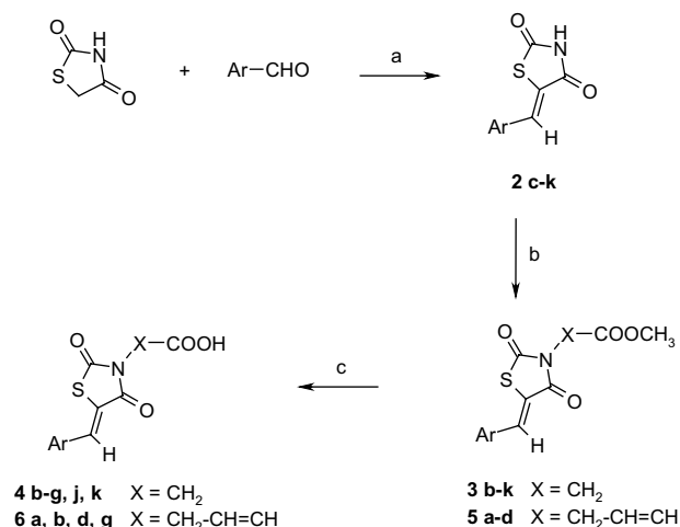
Scheme 1. Reagents: (a) C 5 H 11 N, refluxing C 2 H 5 OH; (b) K 2 CO 3 , acetone, BrCH 2 COOCH 3 or BrCH 2 CH=CHCOOCH 3 ; (c) AcOH, HCl, reflux.
