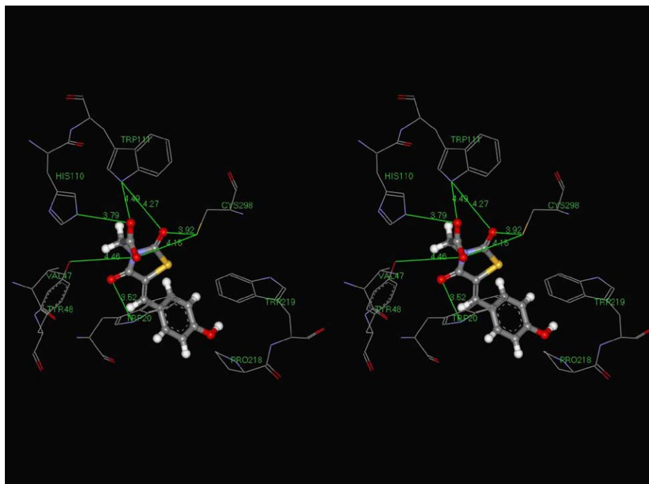
Figure 6. Possibilities of hydrogen bond interactions of docked inhibitor 4g in the ALR2 active site.
