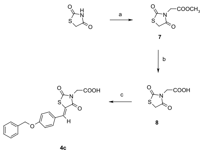
Scheme 2. Reagents: (a) K 2 CO 3 , acetone, BrCH 2 COOCH 3 ; (b) AcOH, HCl, reflux; (c) 4-benzyloxybenzaldehyde, C 5 H 11 N, refluxing C 2 H 5 OH.
