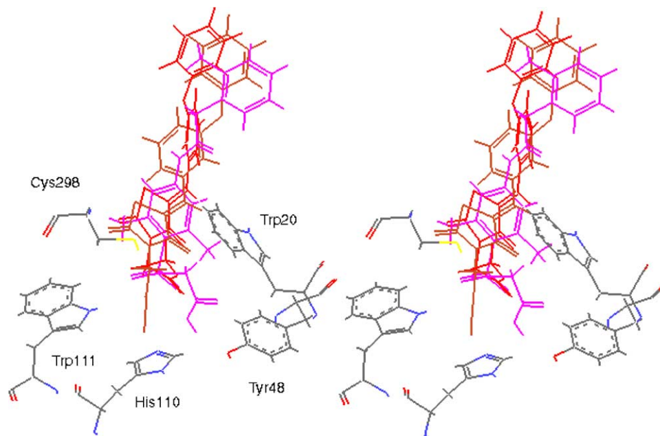
Figure 4. Superposition of docked structures of compounds 3a (red) and 4a (orange) with the bound conformation structure of Idd384 (purple) (relaxed stereo view).
